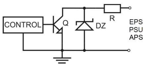
Fig. 5. Electrical diagram of OC outputs.
